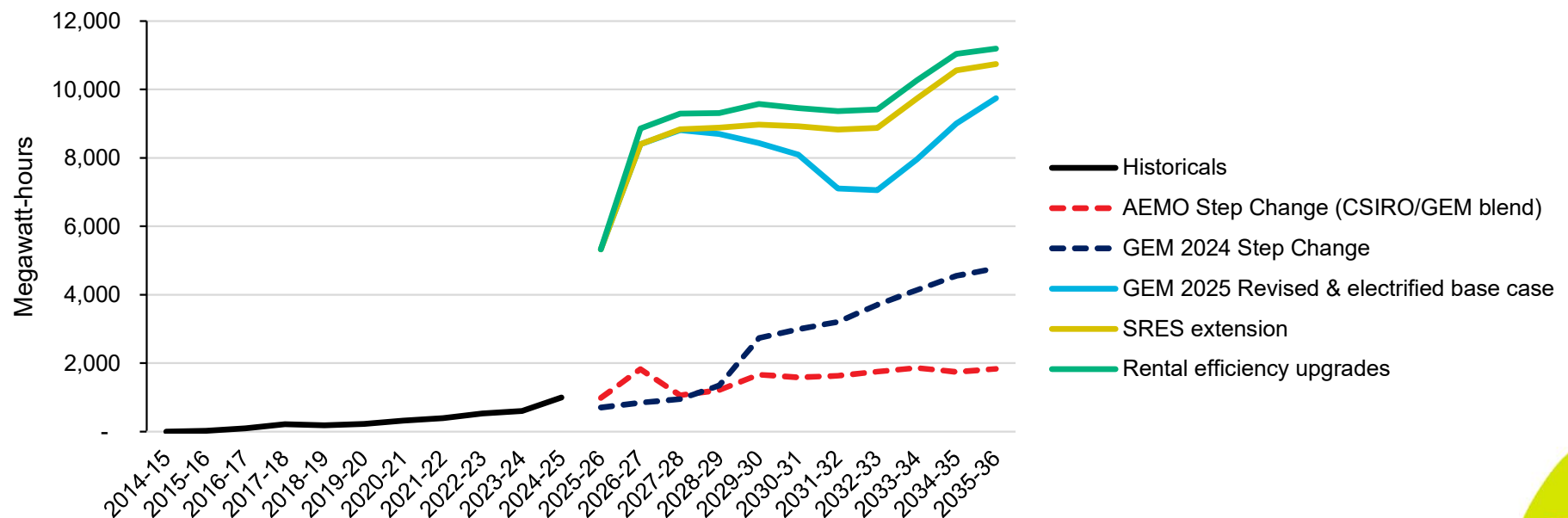
Annual additions of small battery capacity –Updated projections relative to prior projections and historicals
